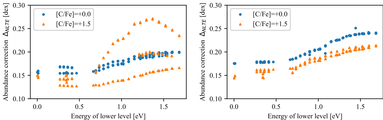
Fig. 12. NLTE abundance corrections for individual G -band lines for model atmospheres with metallicity [\text{Fe}/\text{H}] = -3.0 (left) and [\text{Fe}/\text{H}] = -4.0 (right) for carbon-to-iron ratios [\text{C}/\text{Fe}] = +0.0, +1.5 .
