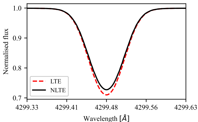
Fig. 7. The LTE and NLTE line profiles of the representative G -band line at 4299.48 Å.
