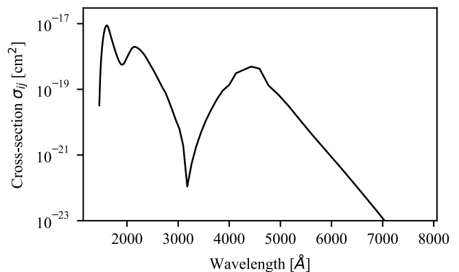
Fig. 5. Cross-section distribution of the photo-dissociation for the energy level at 2.45 eV ( 19777.31 \text{ cm}^{-1} ) with the following configuration: electronic state X^2\Pi with quantum numbers v = 0 and J = 40 .
