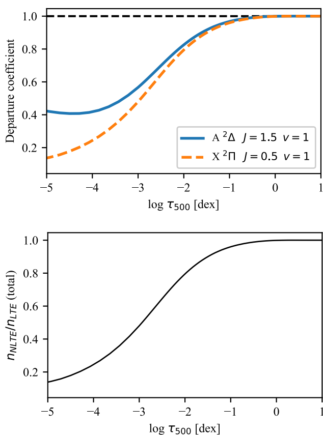
Fig. 8. Top panel: The departure coefficients for the upper level of the transition A^2\Delta with E = 3.2 eV, J = 1.5 and v = 1 and the lower level X^2\Pi with E = 0.3 eV, J = 0.5 and v = 1 . The dashed black line indicates the departure coefficient for a thermalised level, for which n_i^{\text{LTE}} = n_i^{\text{NLTE}} holds true. Bottom panel: Ratio of the total CH number density in NLTE to the total CH number density in LTE.
