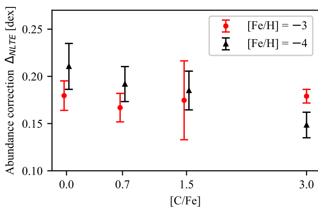
Fig. 11. NLTE abundance corrections for metal-poor carbon-enhanced model atmospheres with metallicities [\text{Fe}/\text{H}] = -3.0 and [\text{Fe}/\text{H}] = -4.0 and carbon-abundance ratios [\text{C}/\text{Fe}] = 0.0, +0.7, +1.5, and +3.0 .
