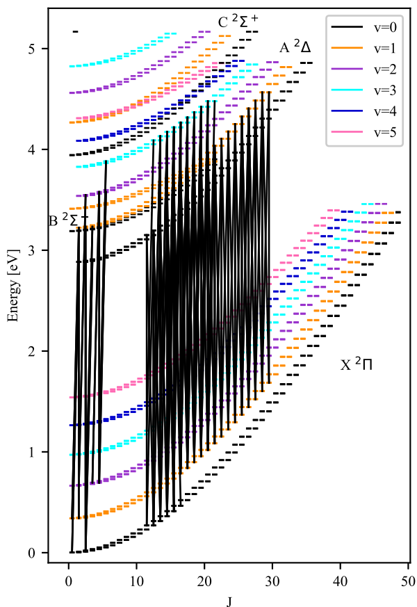
Fig. 2. Energy levels included in the CH molecule model with specified rotational quantum number J and vibrational quantum number v . The black lines indicate the bound-bound transitions between the electronic states A^2\Delta and X^2\Pi that give rise to the molecular G -band lines in wavelength range 4297 - 4303 Å.
