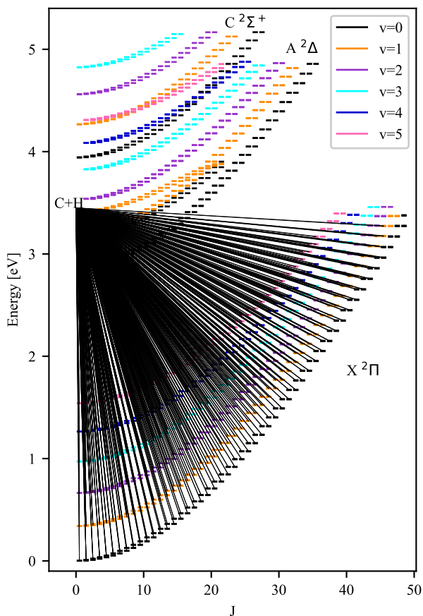
Fig. 4. The black lines indicate the transitions for the photo-dissociation reactions with the dissociation energy of 3.45 eV.
