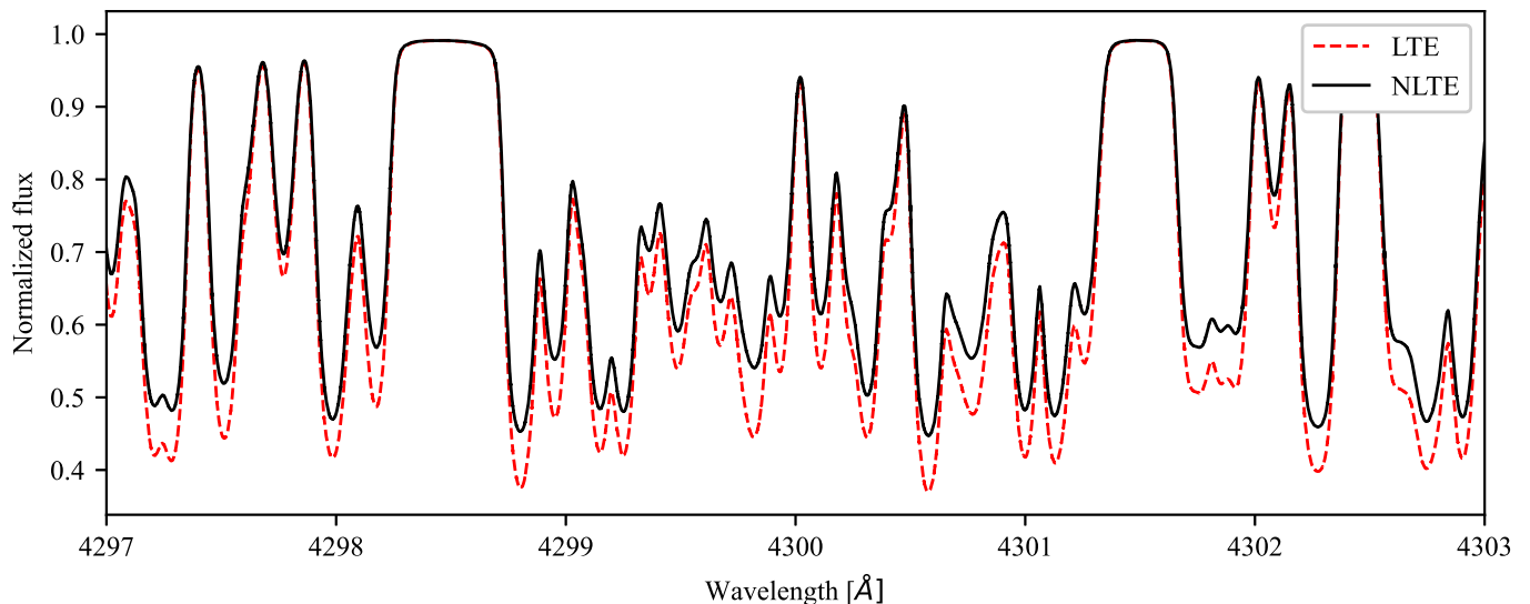
Fig. 6. LTE and NLTE spectra in the region of the CH G -band, computed using the model atmosphere with a solar carbon abundance of A(C)=8.43 .
