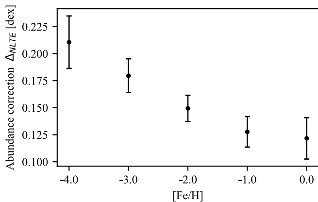
Fig. 10. NLTE abundance corrections for model atmospheres with T_{\text{eff}} = 4500 K and \log g = 2.0 with different metallicities, [\text{Fe}/\text{H}] .
