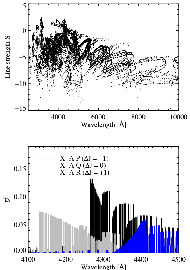
Fig. 1. Top panel: Distribution of line strengths in the entire CH system. Only transitions with strengths greater than S = -5 are included in the NLTE model molecule. Bottom panel: The X-A spectrum of the CH molecule around the wavelength of \sim 4300 Å. The P-, Q-, and R-branches are indicated. The strongest feature in this range, corresponding to J' - J'' = 0 (vibrational transition accompanied by a rotational transition) is the astrophysically famous 'G-band'.
