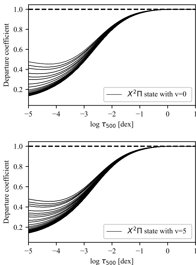
Fig. 9. Departure coefficients of levels in the ground state X^2\Pi with vibrational quantum number \nu = 0 (top) and \nu = 5 (bottom), respectively.
